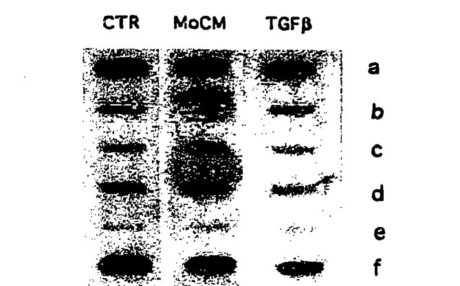
Fig. 3. Nuclear run-on assay performed on control, MoCM- and TGF \beta -treated Hep 3B cells. Plasmids were fixed to nitrocellulose filters and hybridized with 1 \times 10^6 cpm/ml of radiolabelled nuclear transcripts. pBR322 was used as background control. (a) \gamma -actin; (b) AGP; (c) RBP; (d) \alpha 1-antitrypsin; (e) pBR322; (f) albumin.
